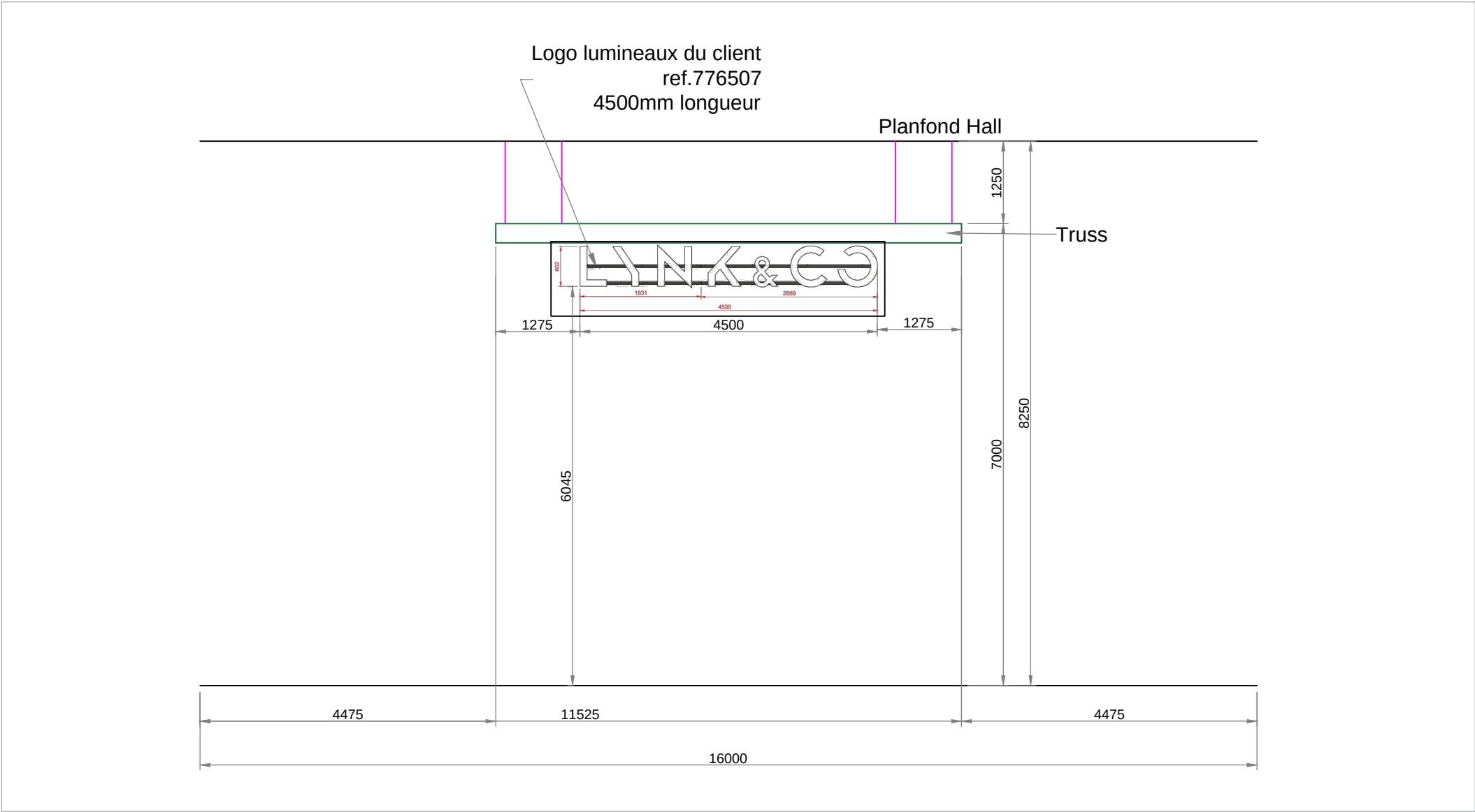
ELEVATION D
